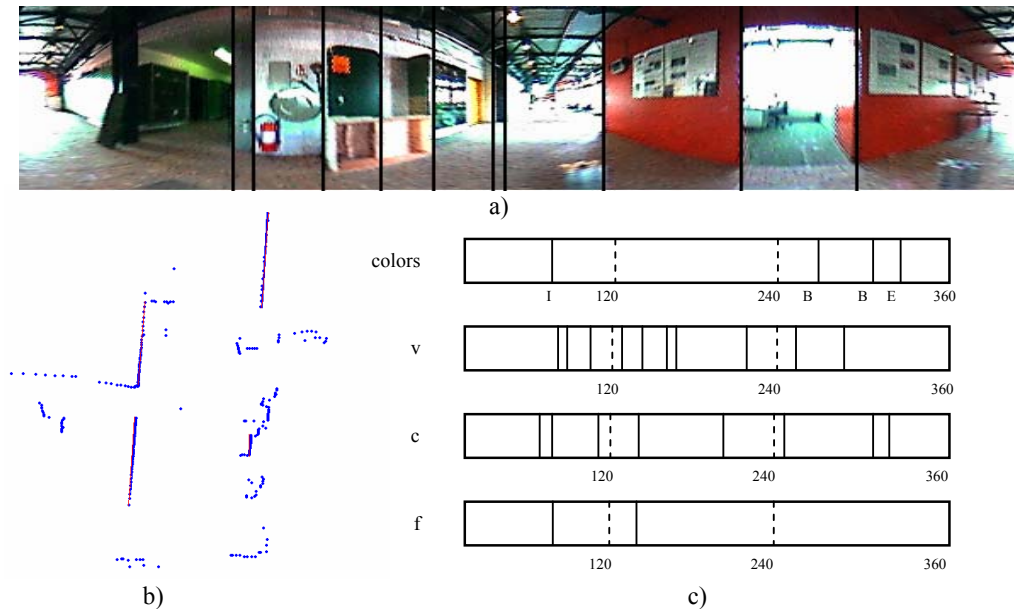
Figure 1: Fingerprint generation. (a) panoramic image with the vertical edges and color patches detection 'v' and color; (b) laser scan with extracted corners 'c'; (c) the first three images depict the position (0 to 360°) of the colors (I-light blue, B- orange and E-light green), vertical edges and corners, respectively. The forth image describes the correspondence between the vertical edges features and the corner features. By regrouping all this results together and by adding the empty space features, the final fingerprint is: clfvnvcvfnvncvnnvcvBnvBccE
